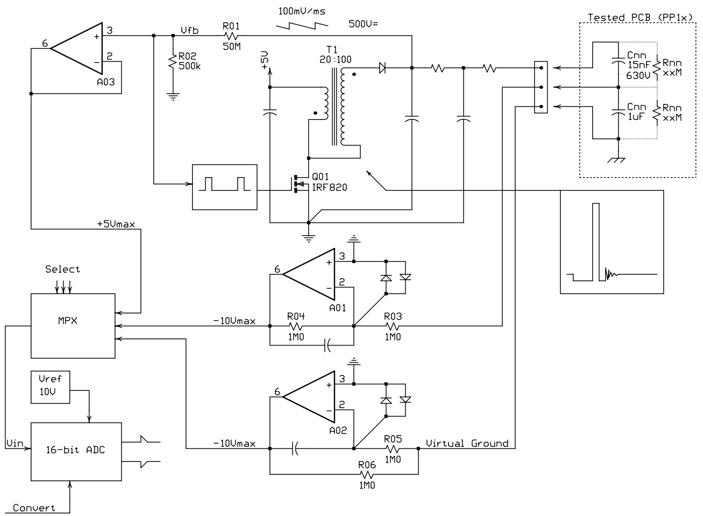
Fig.2 : High-Voltage test
