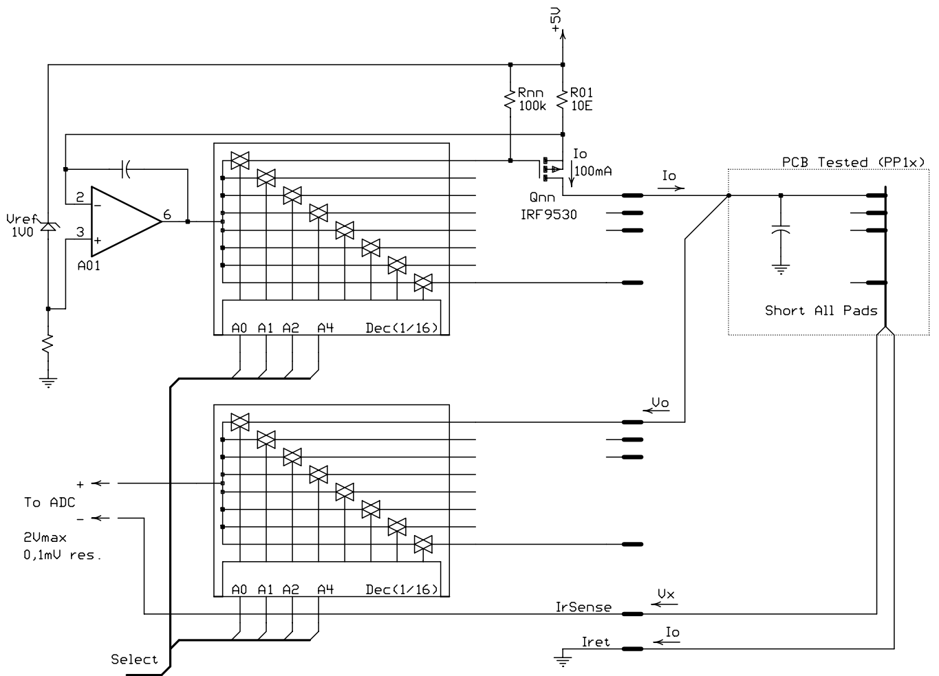
Fig.3 : Line Resistance test
