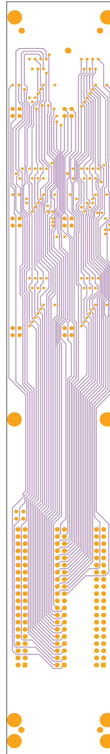
Third Layer
