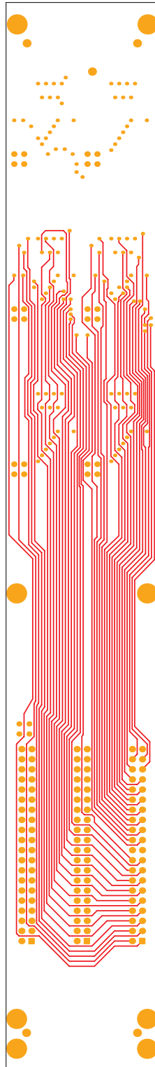
Second Layer
