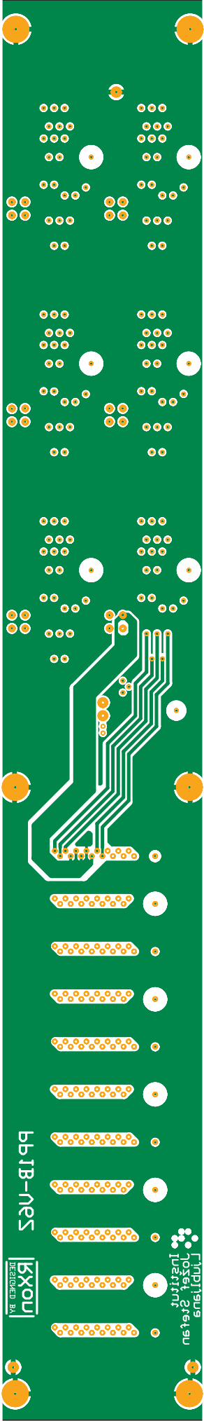
Layer 8 (Bottom + Shield)
