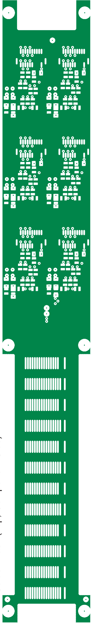
Solder Mask (Top, Component Side)
