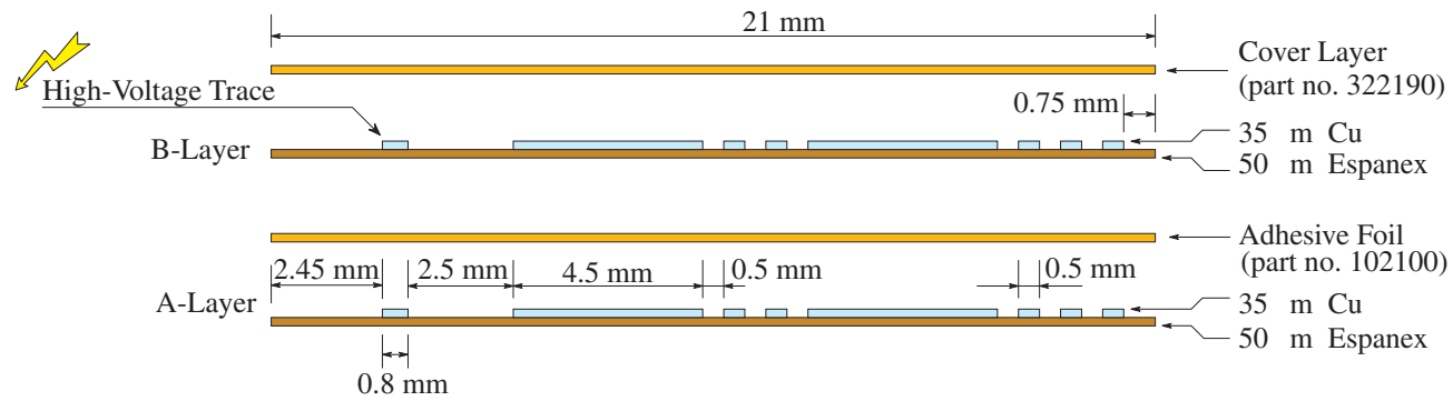
Side view of the tape left-end (1 of 12 shown)
