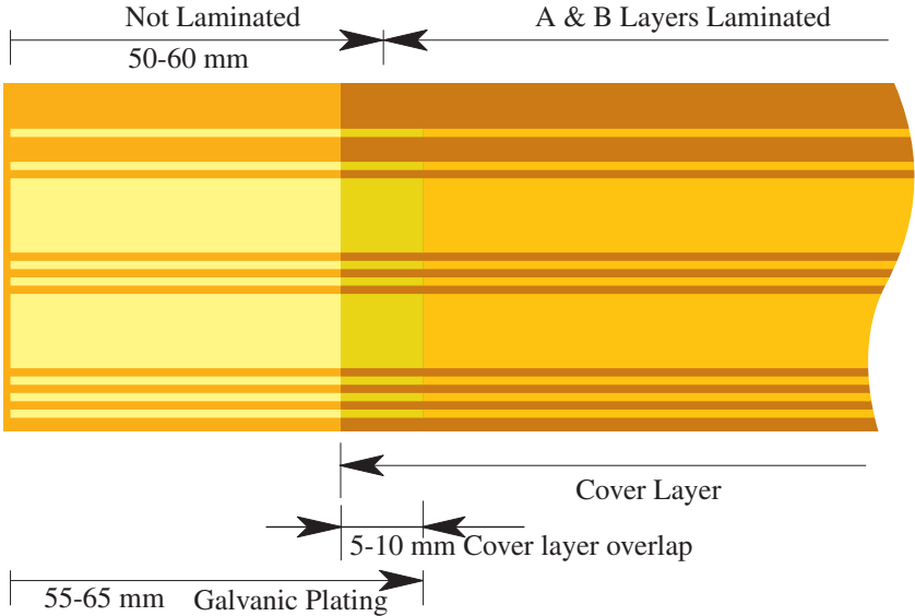
Top view of the tape left-end (1 of 12 shown) ; same galvanic plating and non-laminated section length on the right side.
