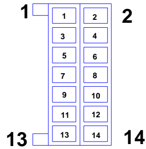
2 x 7 Housing
