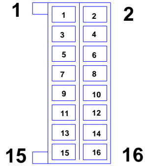
2 x 8 Housing
