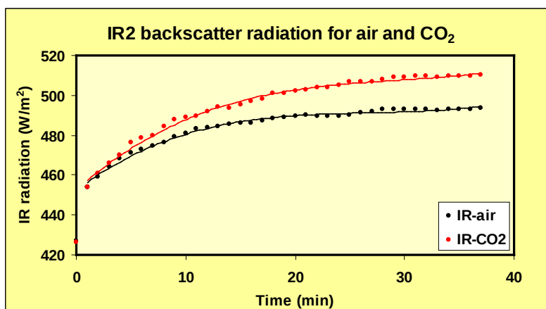
Figure 9. Backscatter (increased IR radiation measured by IR2), received by the rear wall of the box, increased 17\text{ W/m}^2 with \text{CO}_2 in the front box. Heating is done with the Al-foil.
