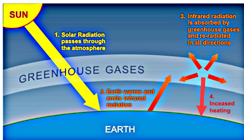
Figure 1. Illustration of the Greenhouse Effect due to greenhouse gases, mainly \text{CO}_2 and water vapor [2].
