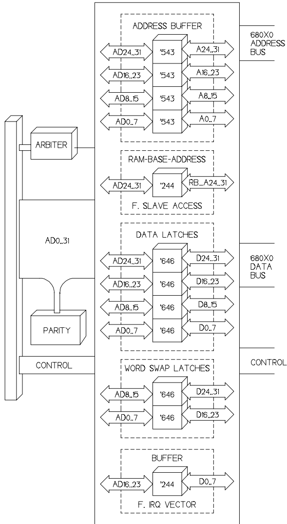
Figure 5. Sample Interface
