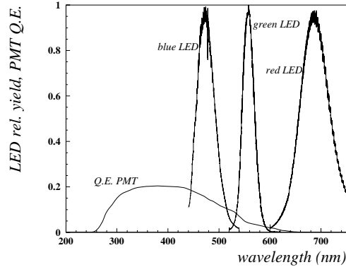
Figure 10: Spectra of three different LED sources.
