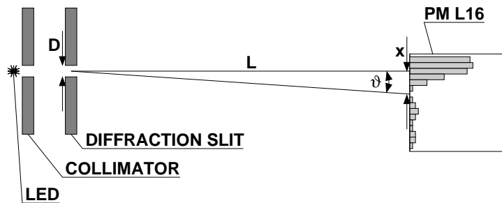
Figure 11: Geometric parameters for the diffraction measurement.
