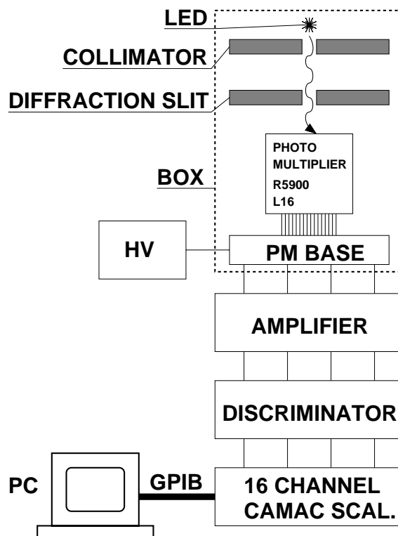
Figure 9: The experimental set-up for measuring diffraction with the L16 PMT.
