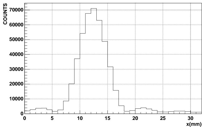
Figure 12: Measured diffraction distribution.
