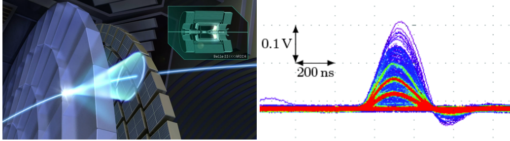
Figure 3: Schematic view of the part of the ARICH detector (left); Response of an HAPD channel to several photons - clear separation between different number of hits is seen in the analog output signal.
