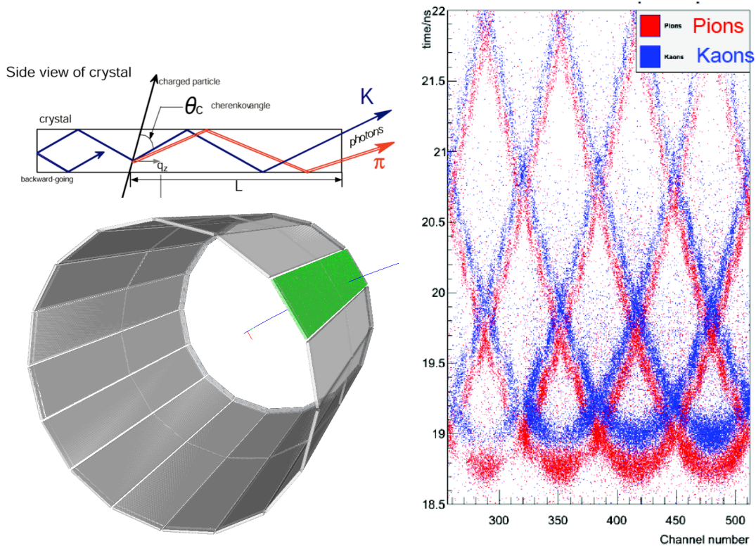
Figure 2: Time Of Propagation counter: principle of measurement (upper left); time of arrival of photons as a function of position (right); 16 quartz bar modules arranged in the Belle II barrel (lower left).
