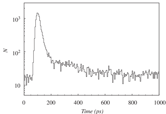
Fig. 2. Time distribution (left) and charge distribution (right) of the response of the 1156 pixel MePhi/PULSAR silicon photomultiplier to the pulsed light source. In the charge distribution the raw spectrum (full lines) and a spectrum for signals within 10 ns window around the peak (dashed) are shown.
