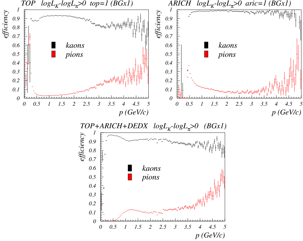
Figure 4: Expected particle identification performance of the Belle II: c\bar{c} events with the expected background; kaon identification efficiency and pion misidentification probability as a function of momentum for TOP (up), ARICH (middle) and combined performance with the dE/dx measurements (bottom).
