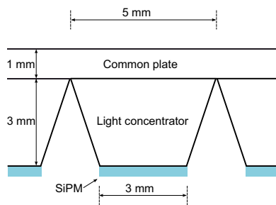
Fig. 1. Light concentrators and SiPMs.
