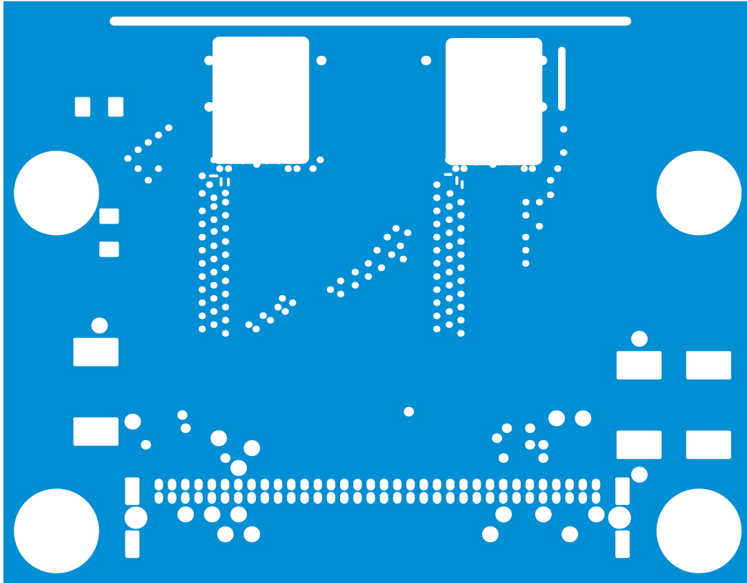
Top Solder Mask
